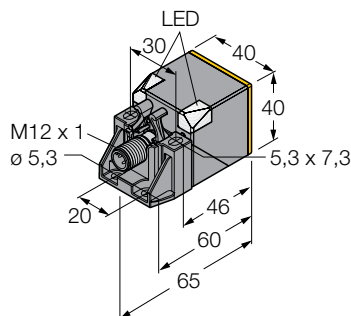
Abb. 5: Dimensions – QV40 design
