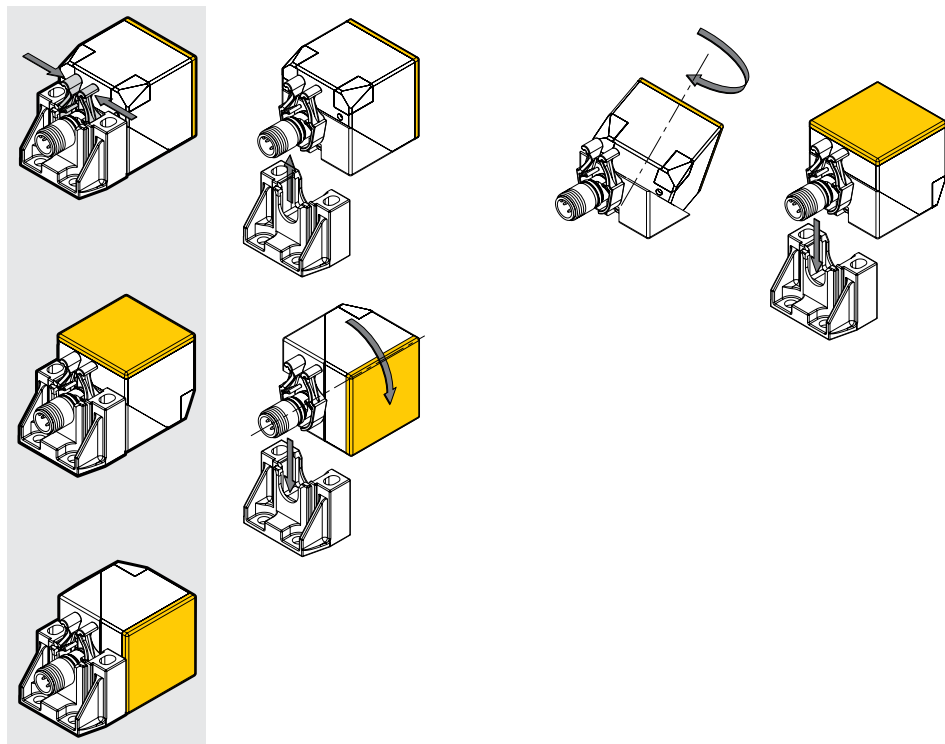
Abb. 13: Positioning the active face
