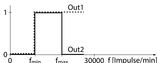
Abb. 6: Output behavior (“Rotational speed monitor” sensor function)
