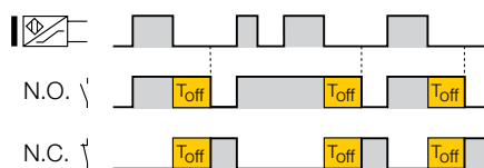
Abb. 8: Switch-off delay
