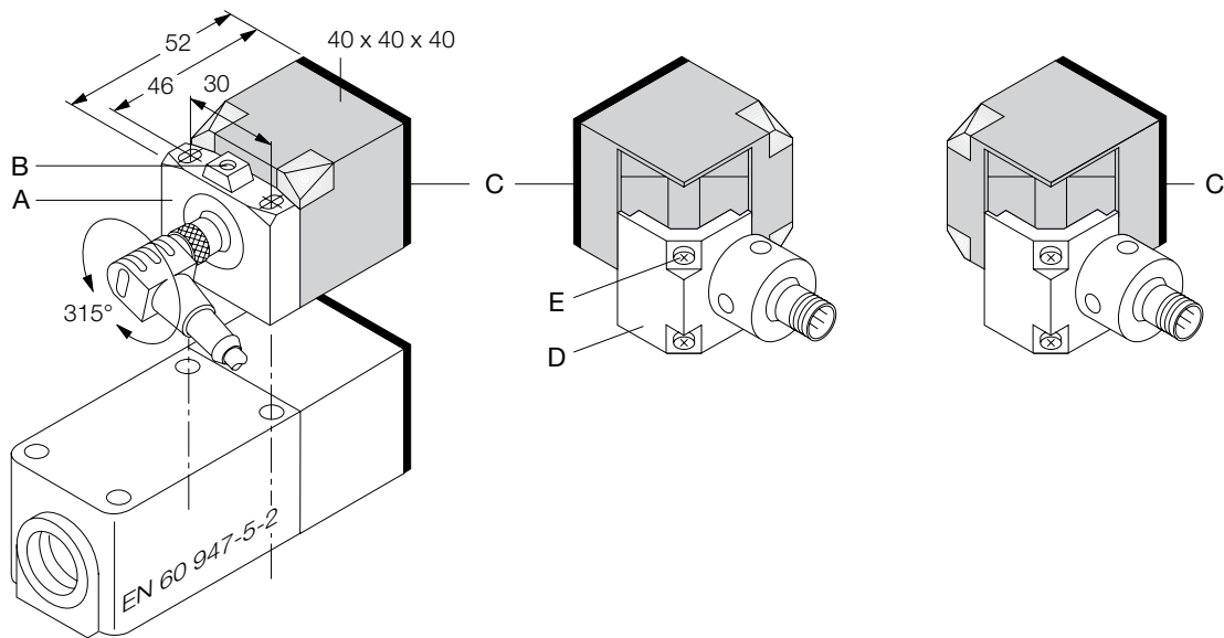
Abb. 14: Positioning the active face
