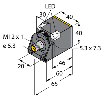
Abb. 4: Dimensions – CK40 design
