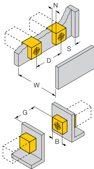
Abb. 11: Minimum mounting distances
