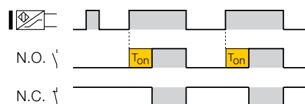
Abb. 7: Switch-on delay
